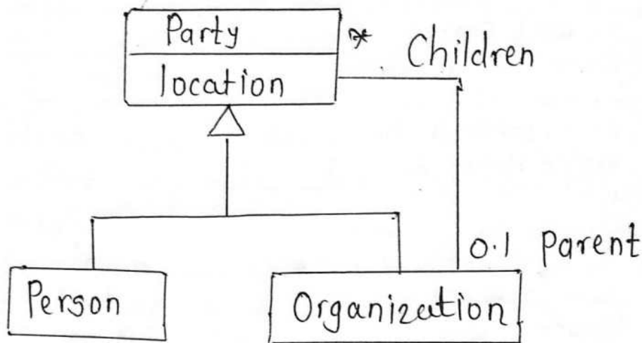
Class diagram of party composition structure
